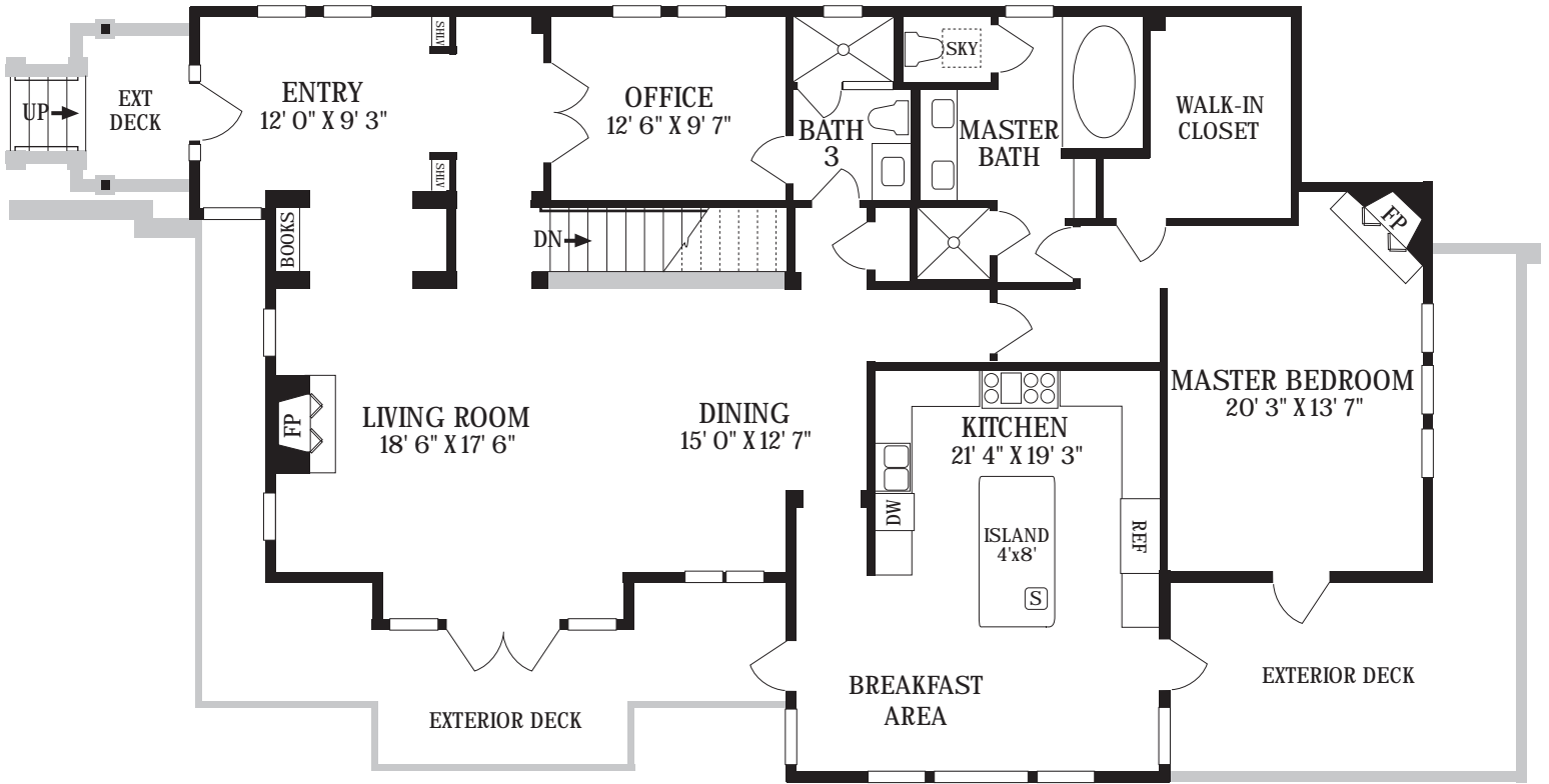
UPPER FLOOR
